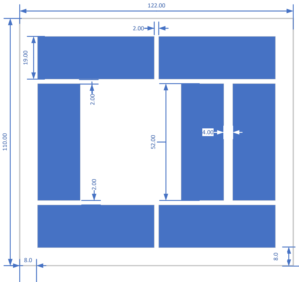
12.2 cm x 11 cm solar panel frame Holds 7 -- 19mm x 52mm panels 8mm edge Tracker package attached in middle area Frame attached to basket using monofilament at each corner
